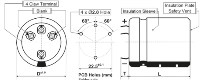
Shape: S (D = 35 ~ 46 mm, long pin T = 6.3 ± 1.0 mm) X (D = 35 ~ 46 mm, short pin T = 4.0 ± 1.0 mm)
