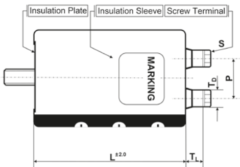
Shape: B = stud bolt (not isolated)
