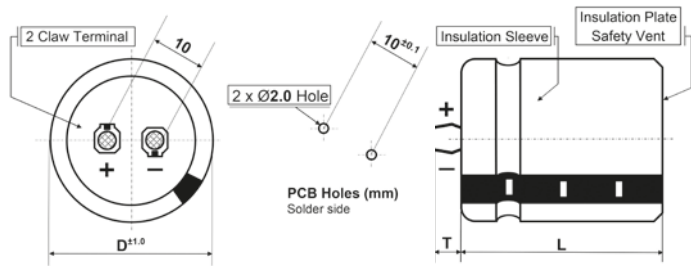
Shape: R (D = 20 ~ 35 mm, long pin T = 6.3 ± 1.0 mm) C (D = 20 ~ 35 mm, short pin T = 4.0 ± 0.5 mm)
