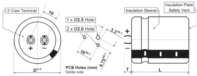
Shape: E (D = 22 ~ 35 mm, T = 4.0 ± 0.5 mm)
