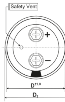
Shape: N with Suffix WC (blank bottom and integrated seating ring for radiator mounting – ØD=77-90 mm)
