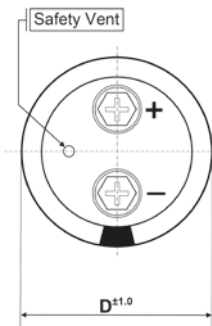
for metal bracket mounting I type: 2 fixing point – Ø D = 36-90 mm Y type: 3 fixing point – Ø D = 51-101 mm X type: 4 fixing point – Ø D = 121 mm
