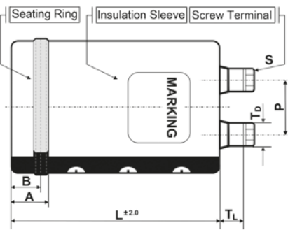
Shape: N with Suffix WC (blank bottom and integrated seating ring for radiator mounting – ØD=77-90 mm)
