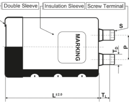
Shape: I, Y, X = bottom double sleeve
