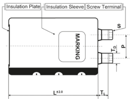
Shape: N (for PBT-Holder – ØD=77-101 mm or for press ring – ØD=64-90 mm or customized)
