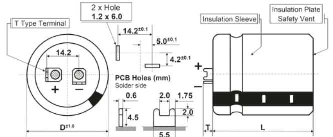
Shape: T (D = 30 ~ 40 mm, T = 4.5 ± 0.5 mm)
