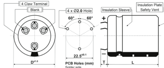
Shape · Form: S (D = 35 ~ 46 mm, long pin T = 6.3 \pm 1.0 mm) X (D = 35 ~ 46 mm, short pin T = 4.0 \pm 1.0 mm)
