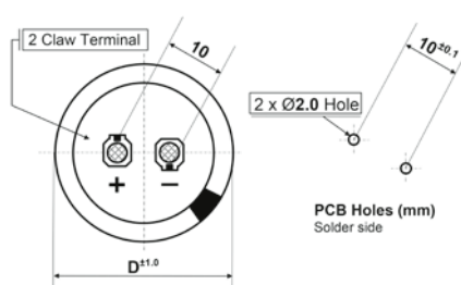
Shape · Form: R (D = 20 ~ 35 mm, long pin T = 6.3 \pm 1.0 mm) C (D = 20 ~ 35 mm, short pin T = 4.0 \pm 0.5 mm)
