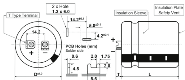
Shape · Form: T (D = 30 ~ 40 mm, T = 4.5 \pm 0.5 mm)
