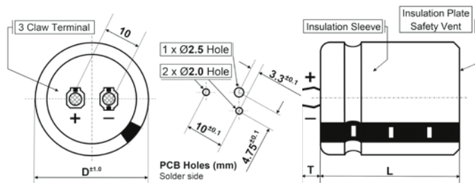
Shape · Form: E (D = 22 ~ 35 mm, T = 4.0 \pm 0.5 mm)
